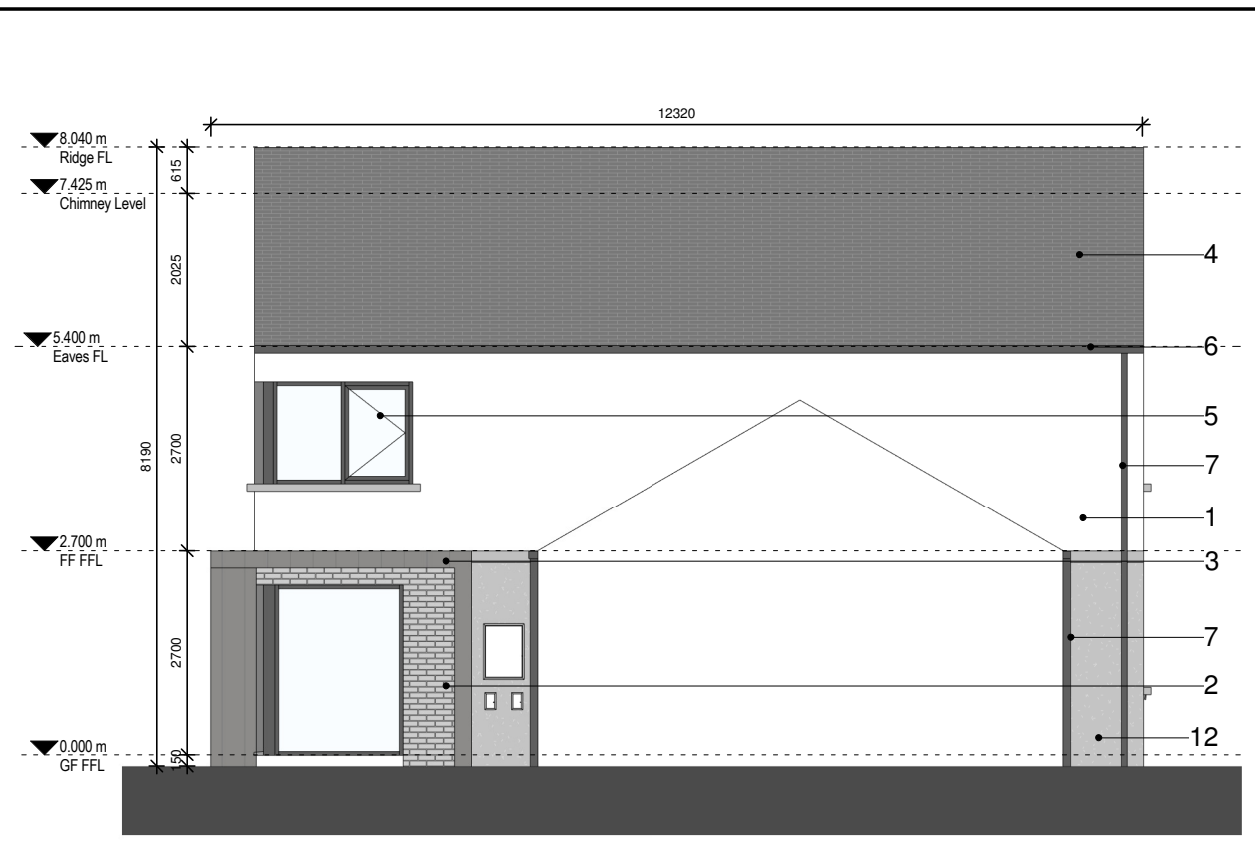
2 05 Side Elevation 1:100 @ A3
