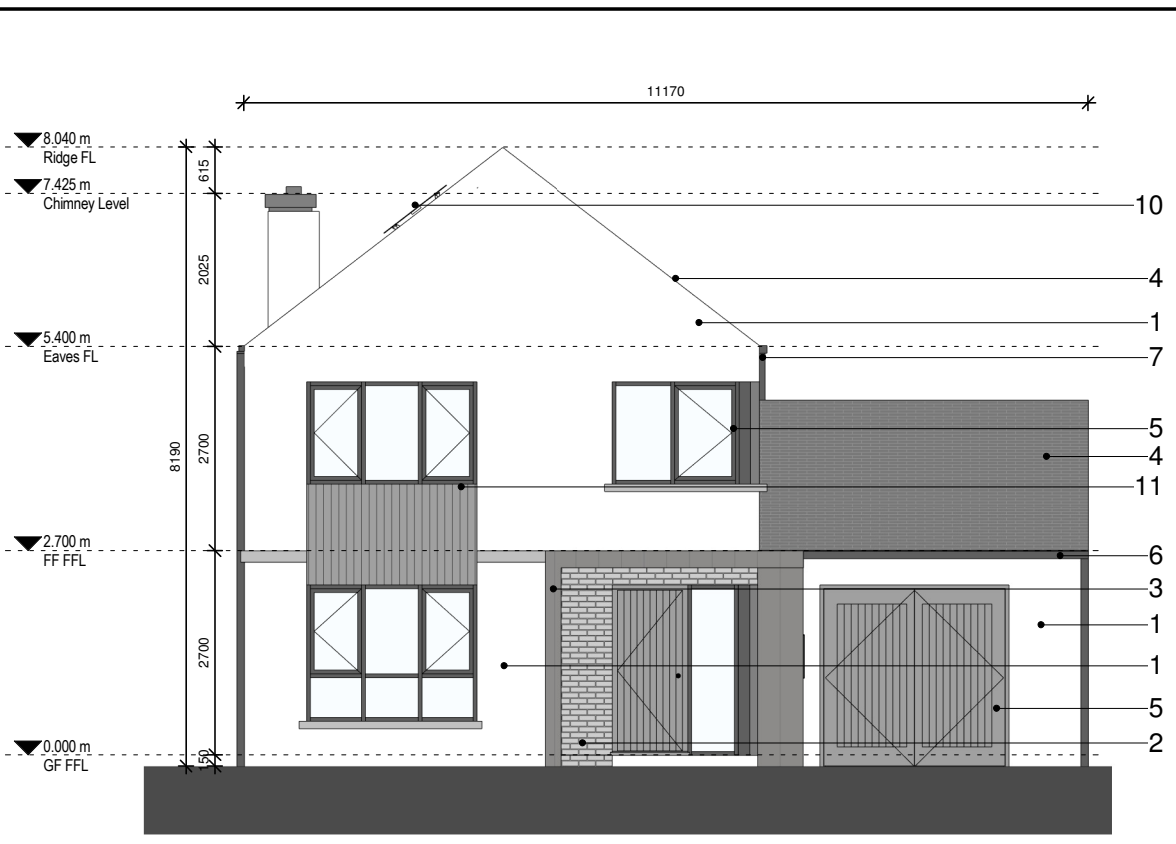
1 04 Front Elevation 1:100 @ A3
