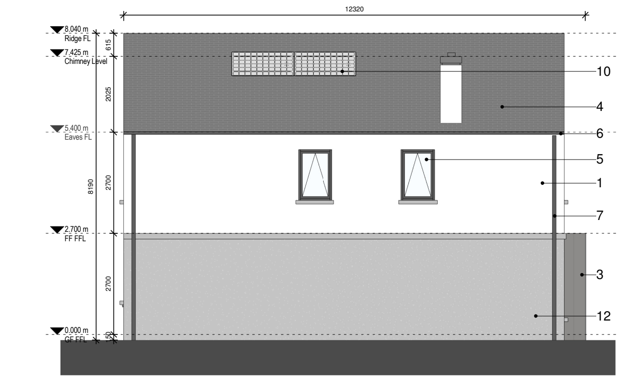
4 07 Side Elevation 1:100 @ A3
